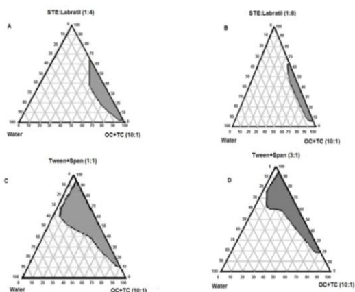
Figure 1. Phase diagrams of novel (A, B) and traditional (C, D) formulations with different ratios of surfactant/cosurfactant
